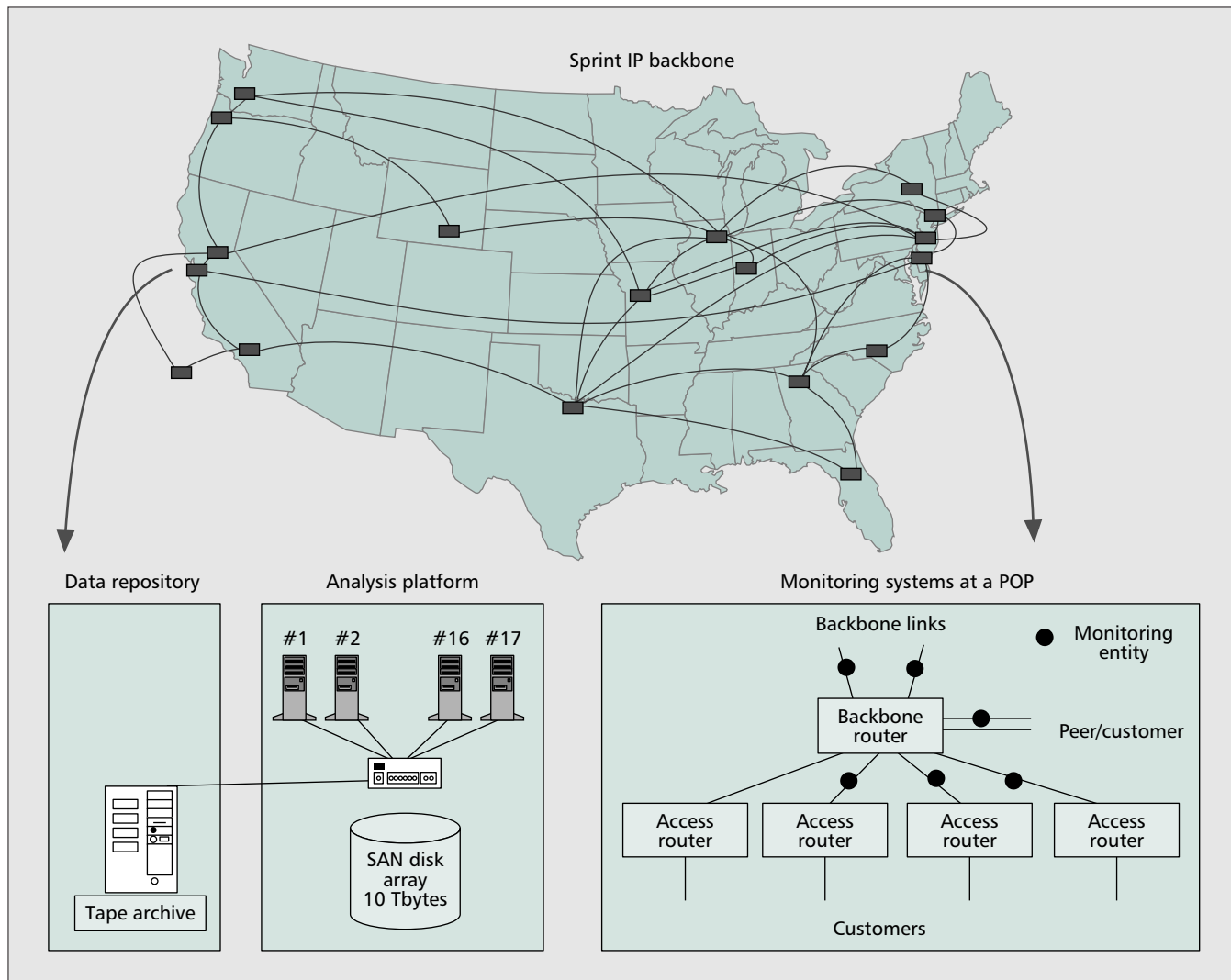
■ Figure 1. The IPMON system in the Sprint IP backbone.
