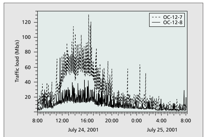
■ Figure 3. A day-long time-series plot from IPMON.
