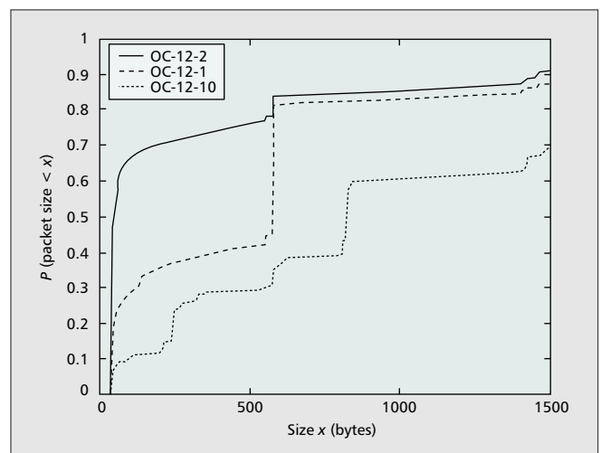
■ Figure 8. Packet size cumulative distribution function.
