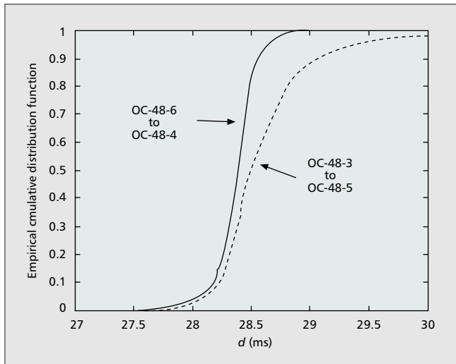
■ Figure 11. Delay distributions.
