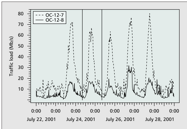
■ Figure 2. A week-long time-series plot from SNMP.
