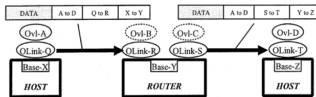
Fig. 9. A single packet traverses the overlay – modifying both outer IP headers at each hop.
