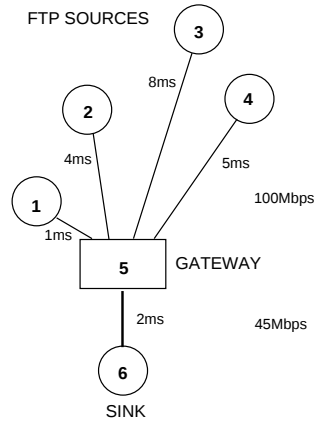
Figure 4: Simulation network.
