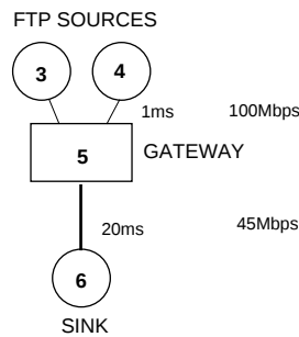
Figure 6: Simulation network.
