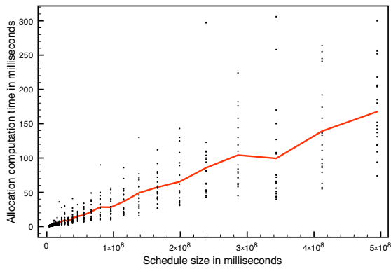
Fig. 10. The amount of time required to find the allocation of jobs, as we vary the size of the schedule.
