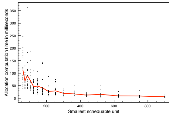
Fig. 12. The amount of time required to find the allocation of jobs, as we vary the size of the smallest scheduable unit.
