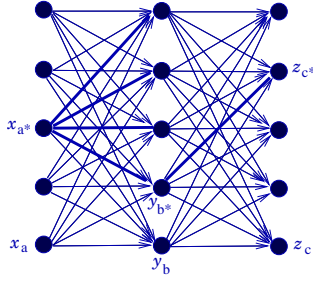
Fig. 2. The lower bound construction of Karger, Koller and Phillips [13]. The edges whose weights are modified are shown as thick lines.
