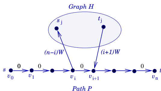
Fig. 1. The main lower bound construction.
