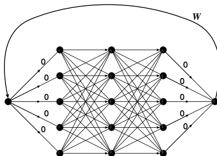
Fig. 3. The lower bound breaks down when we add a useless loop.
