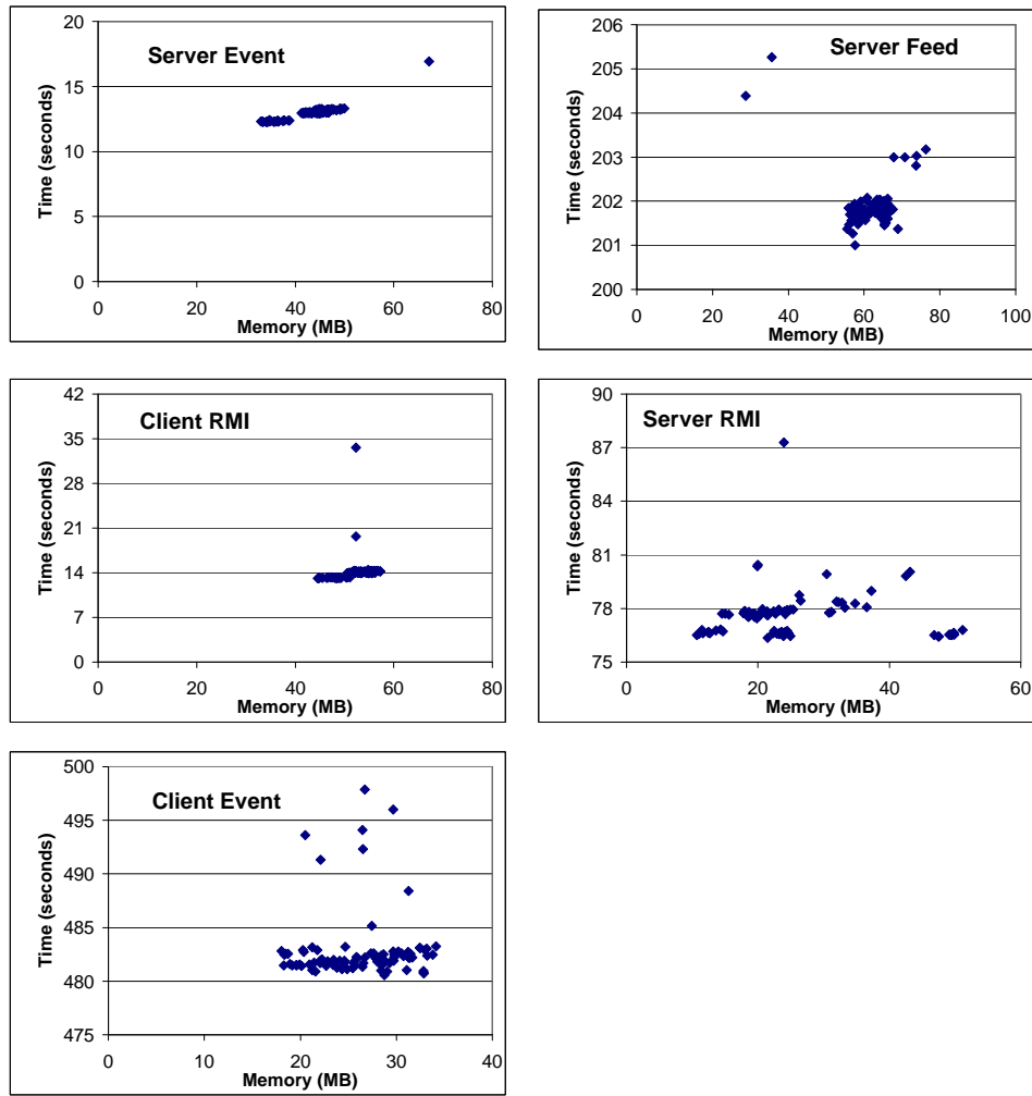
Figure 18. Interface verification performance for vr1–vr100 with JPF
