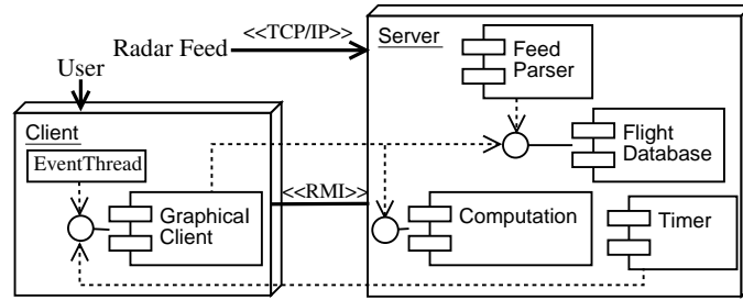
Figure 2. TSAFE architecture.
