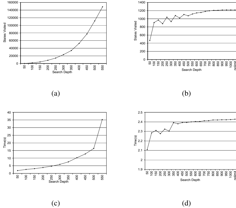
Figure 20. JPF performance using actual controller instance ((a),(c)) and instances of the controller interface as stubs ((b),(d))
