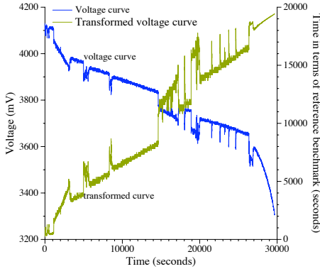
Figure 3: Voltage curve and transformed voltage curve for “real.load.5”
