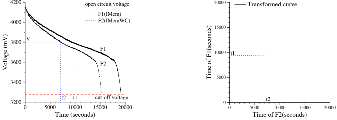
Figure 1: Timing relationship between two voltage curves of constant workloads. F_1 is the curve of the workload that is generated by repeatedly running benchmark “IMem”. And F_2 is the curve of benchmark “IMemWC”. The left graph shows that for some voltage value V , F_1 reaches V at time t_1 and F_2 reaches V at time t_2 . The right graph shows the linear relationship between t_1 and t_2 for any V .
