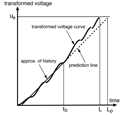
Figure 4: Prediction error calculation
