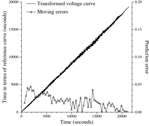
Figure 6: Transformed voltage curve and moving errors for the Reg, constant workload, benchmark. The left y -axis is the transformed voltage in terms of reference curve time. The right one shows the value of errors. We set the maximum to be 20%.
