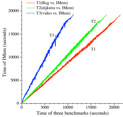
Figure 2: Timing relationship: \Gamma function. This graph plots the \Gamma functions for three pairs of constant workloads: “Reg” and “IMem”, “dijkstra” and “IMem”, “video” and “IMem”. Since “IMem” is common for all three curves, we can plot them in the same graph.
