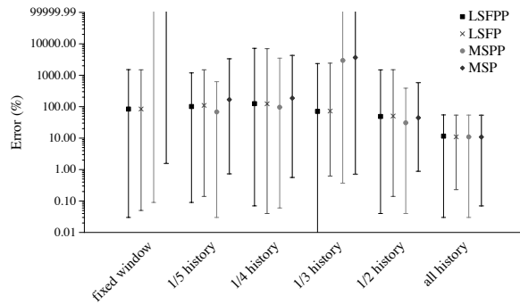
Figure 8: Prediction performance for different history size. This figure shows the mean, max and minimum of “moving errors” of the 4 methods for real.load.5 benchmark, using different history size: fixed window, 1/5, 1/4, 1/3, 1/2, all history. Values out of range are clipped.
