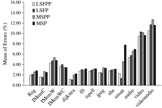
Figure 7: Average prediction errors for constant workloads
