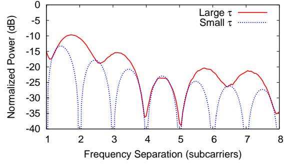
Figure 3: An example of the cross-band interference. X-axis is the frequency separation to the interferer, Y-axis is the normalized power.
