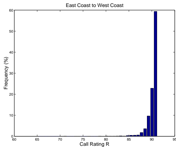
Figure 10: Distribution of voice call ratings (excluding the failure event)
