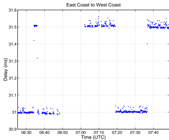
Figure 4: Average delay during the failure. Each dot corresponds to a five-second interval
