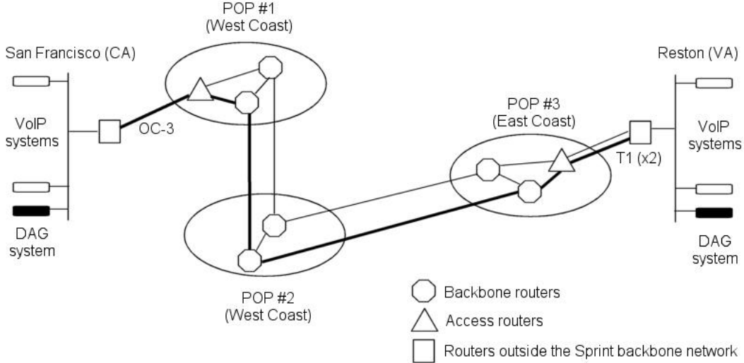
Figure 1: Topology of the active measurement systems (the thick lines indicate the primary path)
