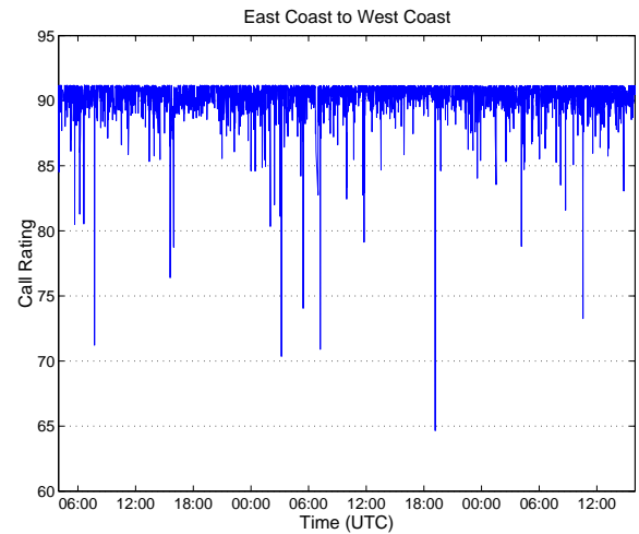
Figure 9: Voice call ratings (excluding the failure event)
