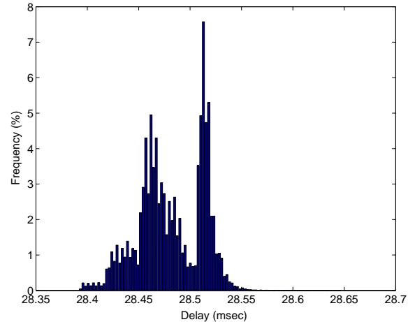
Figure 2: Passive measurements: distribution of the one-way transmission delay between East and West Coast of the U.S.
