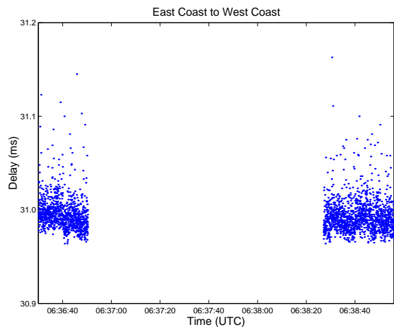
Figure 6: One-way delay of voice packets during the first 100% loss period
