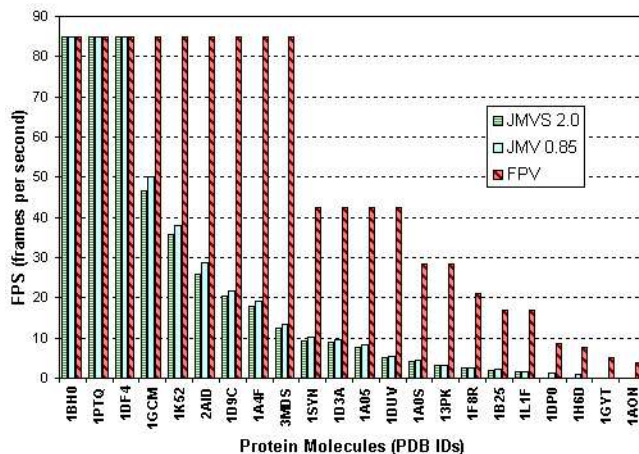
Figure 13: Rendering Speed for the VDW Model
