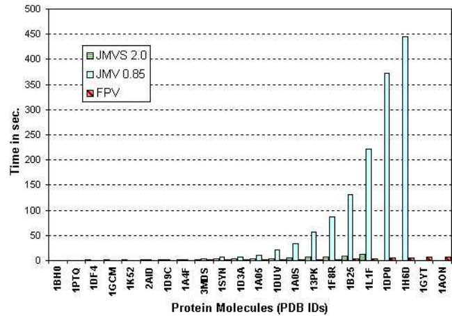
Figure 17: Scene Building Times for the VDW Model
