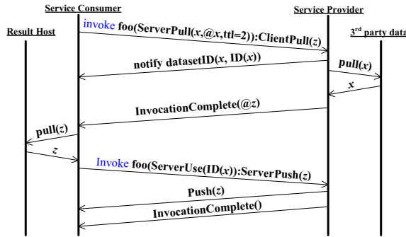
Figure 5: Invocation Using ServerUse
