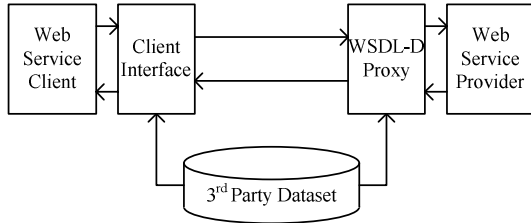
Figure 6: Architecture of the WSDL-D prototype
