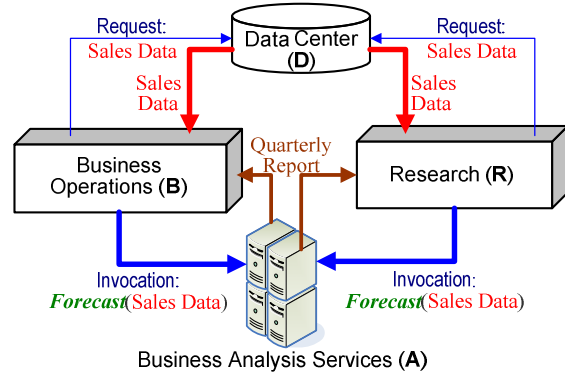
Figure 1: A business application scenario
