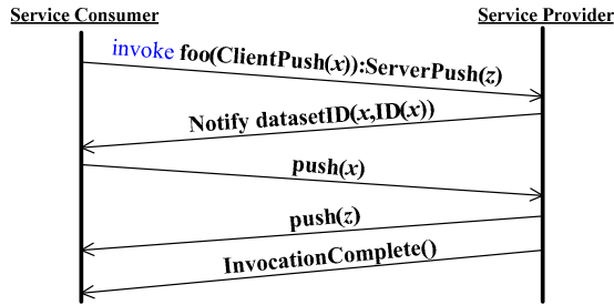
Figure 3: Invocation using ClientPush
