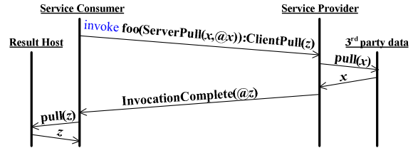
Figure 4: Invocation Using ServerPull
