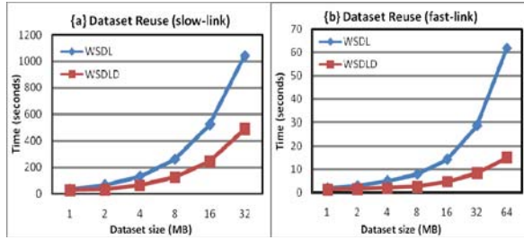
Figure 8: Service execution time (the dataset stored at the service provider)
