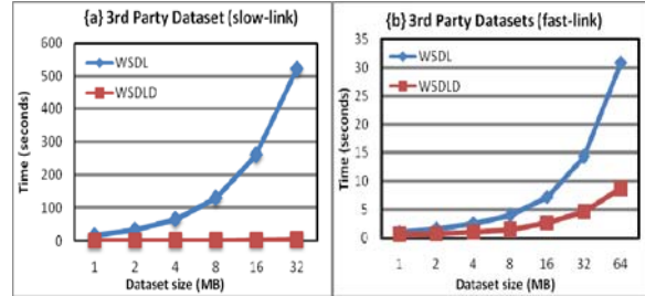
Figure 7: Service execution time (the dataset at a 3rd party host)
