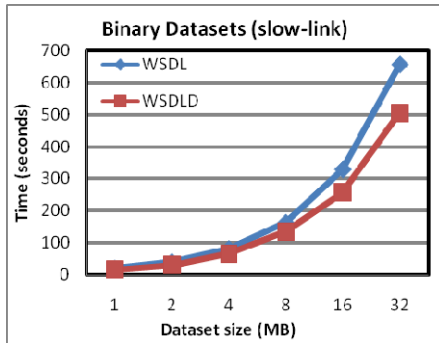
Figure 9: Invocations with binary datasets
