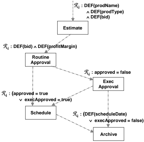
Figure 3: Simple ruleset that is \gamma_1 -safe
