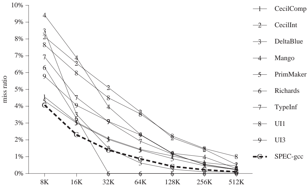
Figure 6. Instruction cache miss ratios of SELF programs (direct-mapped cache, 32-byte lines)
