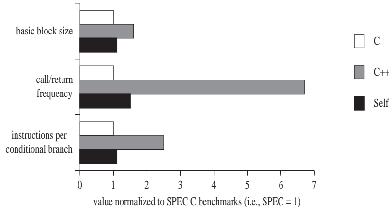
Figure 3. Differences between SELF/C++ and the SPEC C programs
