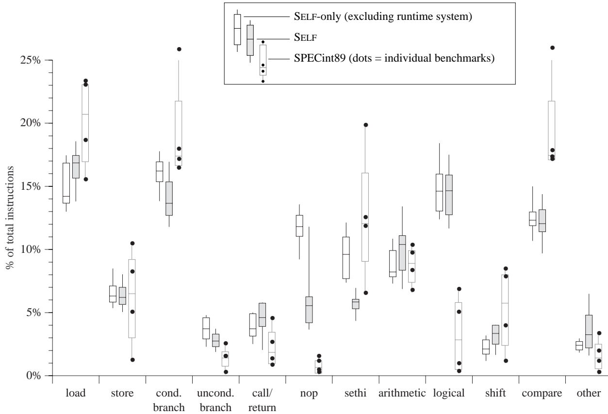
Figure 1. Dynamic instruction usage of SPEC integer benchmarks and SELF-93 benchmarks
