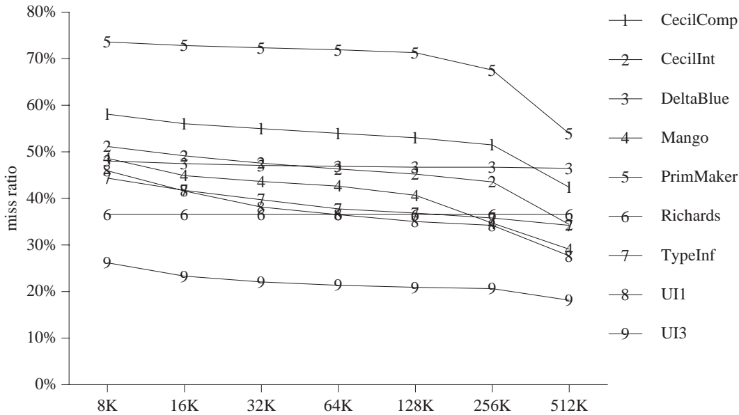
Figure 9. Write miss ratio (direct-mapped, 32-byte lines, write-noallocate)
