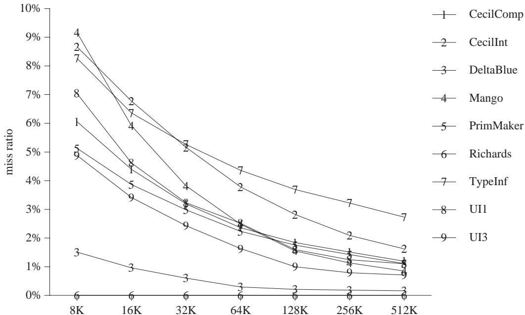
Figure 7. Data cache read misses (direct-mapped, 32-byte lines, write-allocate with subblock placement)
