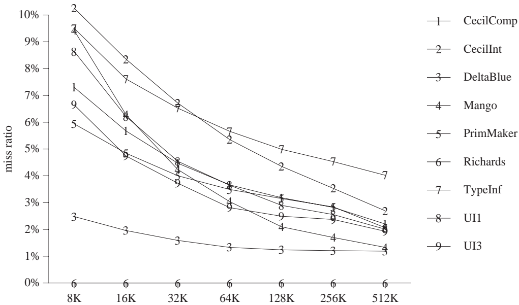
Figure 8. Data read misses (direct-mapped, 32-byte lines, write-noallocate)
