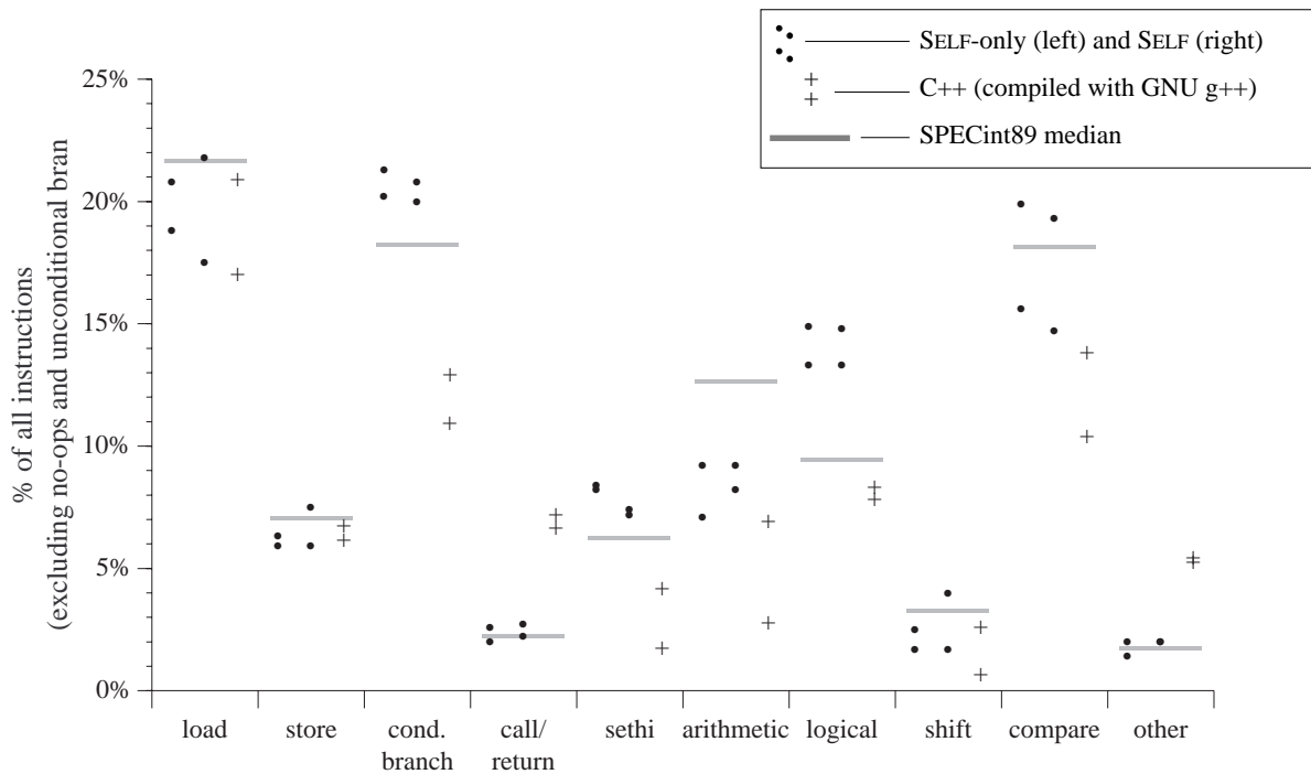
Figure 4. Instruction mix for SELF and C++ on Richards and DeltaBlue benchmarks
