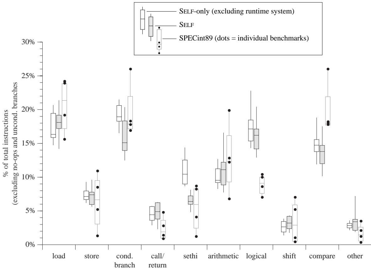
Figure 2. Dynamic instruction usage of SPEC89 integer benchmarks and SELF-93 benchmarks (adjusted)
