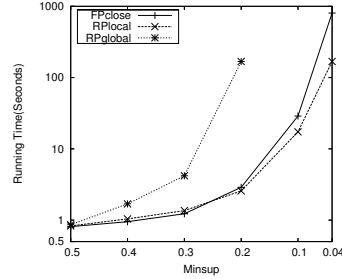
Fig. 18. Running Time w.r.t. min\_sup , Pumsb_star Data Set
