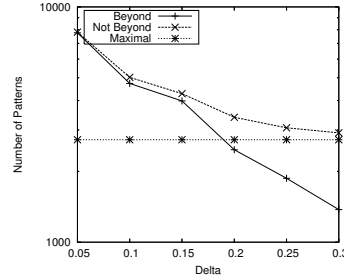
Fig. 26. Number of Output Patterns, Accidents Data Set
