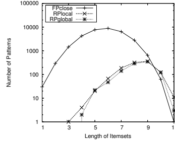
Fig. 20. Distribution of Patterns w.r.t. Pattern Length, Accident Data Set
