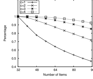
Fig. 9. Simulation Results: Percentage of Closed Pruning achieved
