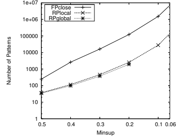
Fig. 14. Number of Output Patterns w.r.t. min\_sup , Pumsb_star Data Set
