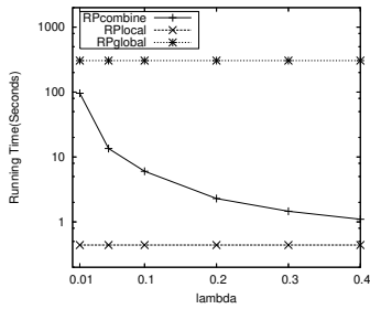
Fig. 25. Running Time w.r.t. \lambda , Chess Data Set
