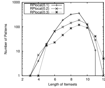
Fig. 22. Distribution of Patterns w.r.t. Pattern Length, Accident Data Set
