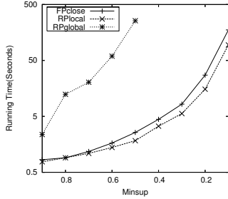
Fig. 17. Running Time w.r.t. min\_sup , Connect Data Set
