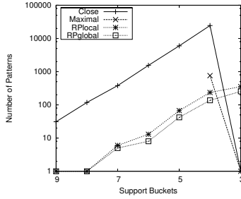
Fig. 21. Distribution of Patterns w.r.t. Support Buckets, Accident Data Set
