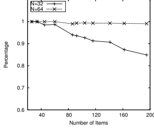
Fig. 8. Percentage of Closed Pruning achieved
