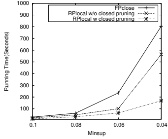
Fig. 19. Running Time w.r.t closed pruning, Pumsb_star Data Set
