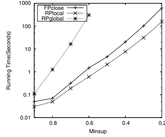
Fig. 16. Running Time w.r.t. min\_sup , Chess Data Set
