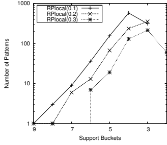
Fig. 23. Number of Output Patterns w.r.t. Support Buckets, Accidents Data Set
