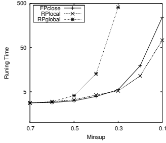
Fig. 15. Running Time w.r.t. min\_sup , Accidents Data Set
