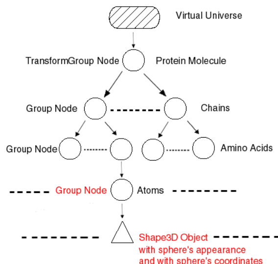
Figure 8: The scene-graph after applying first technique.
