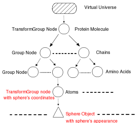
Figure 7: A fragment of an intuitive scene-graph for VDW model.
