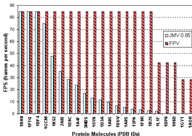
Figure 16: Rendering Speed for the Ribbon Model
