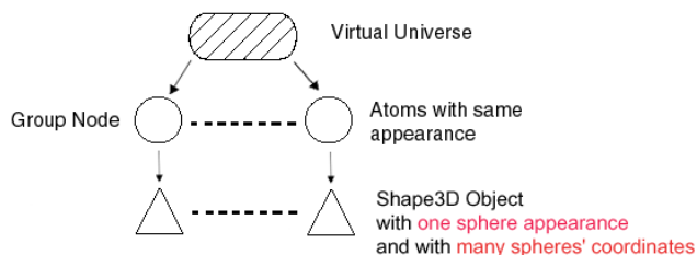
Figure 9: The scene-graph after applying the second technique.
