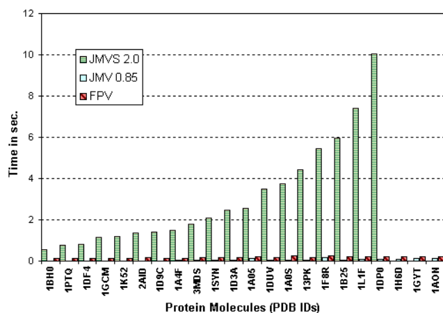
Figure 18: Scene Building Times for the Bonds Model
