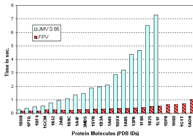
Figure 19: Scene Building Times for the Ribbon Model
