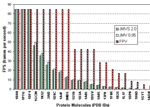
Figure 13: Rendering Speed for the VDW Model
