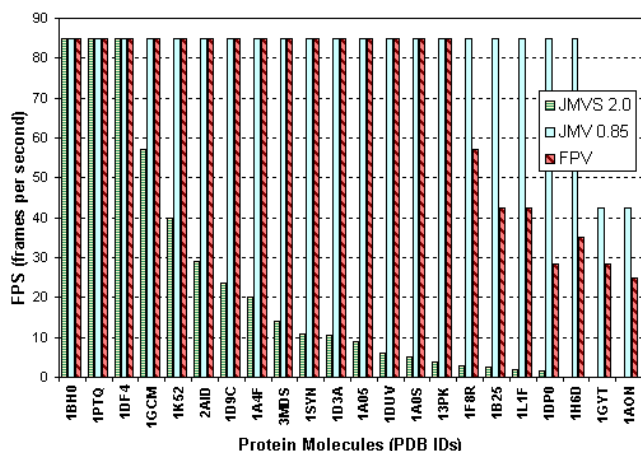
Figure 15: Rendering Speed for the Bonds Model
