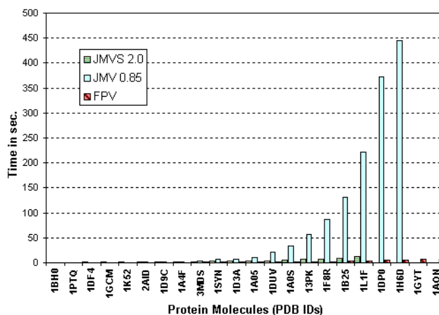
Figure 17: Scene Building Times for the VDW Model
