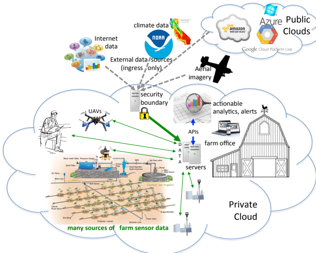
Figure 1: SMARTFARM Vision (left) and the SMARTFARM Software Architecture (right)
