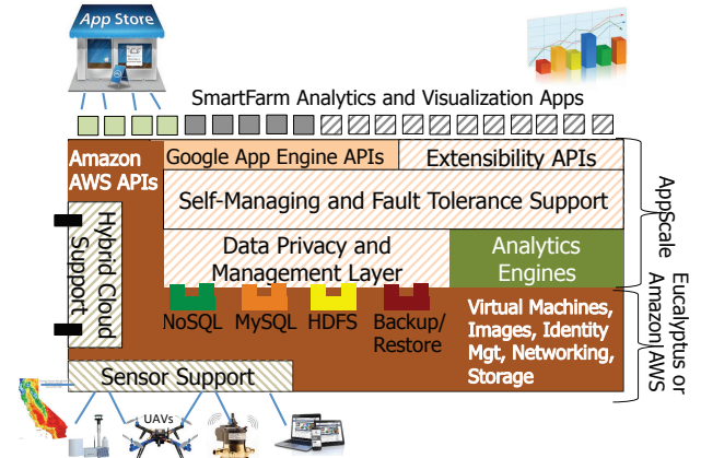
Figure 1: SMARTFARM Vision (left) and the SMARTFARM Software Architecture (right)
