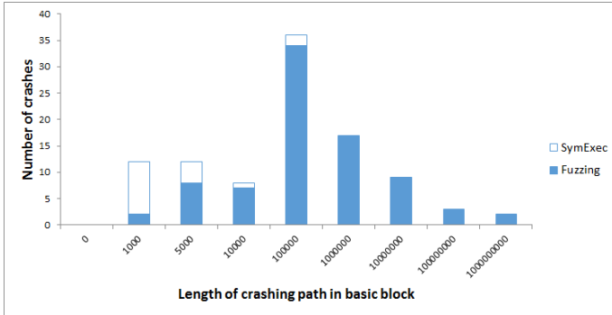
Fig. 1. Length of crashing paths discovered by fuzzing vs. dynamic symbolic execution.
