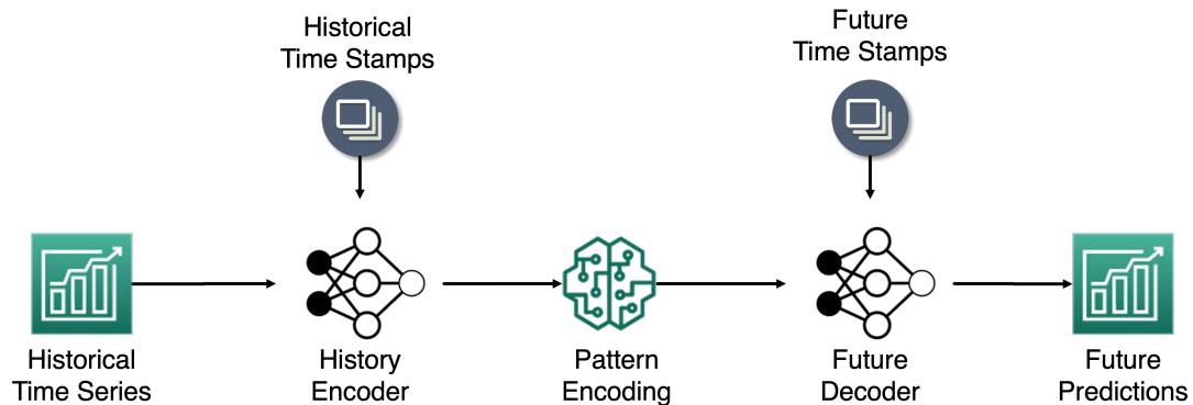
Figure 1.2: General structure of forecasting models. Besides historical time series, the time stamps of the past and the future can also be helpful.
